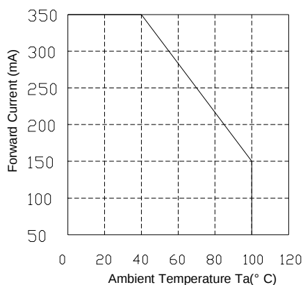
Derating
