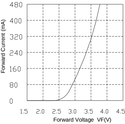
Forward Voltage vs. Forward Current (Ta=25 °C)
